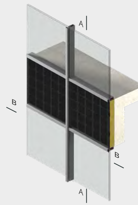
SPANDREL OF CURTAIN WALL WITH COVER CAPS
