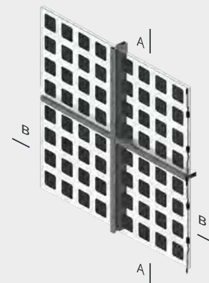
CURTAIN WALL WITH CONCEALMENT CAPS
